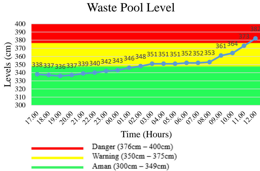
Figure 10. Data recorded in the waste pond level monitoring system
